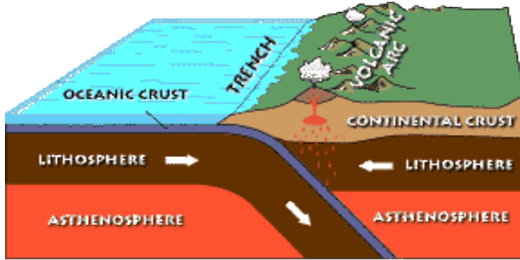
Convergent plate boundary Subduction zone
