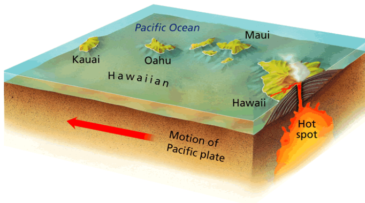
Hot spots (Hawaii)
