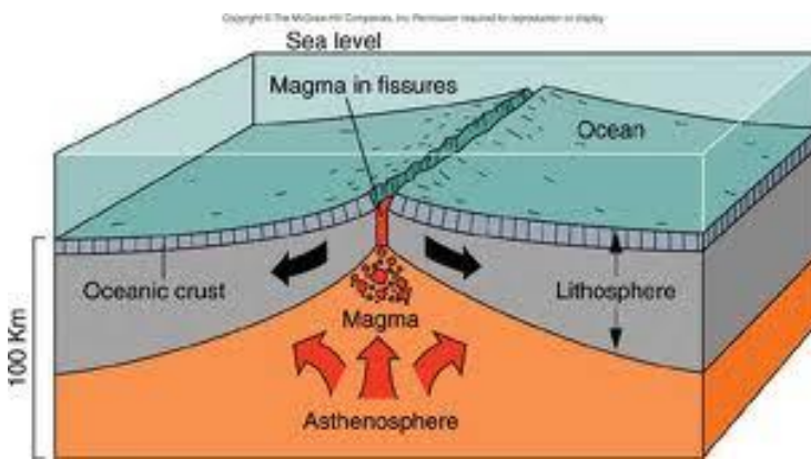
Divergent plate boundary Mid-ocean ridge
